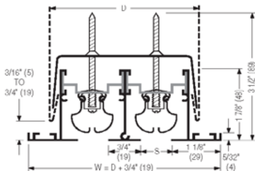
Flange Frame / Concealed Mounting
