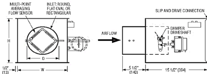
Nailor Industries Single Duct Terminal Unit Nailor model# P3101 (Pneumatic)
